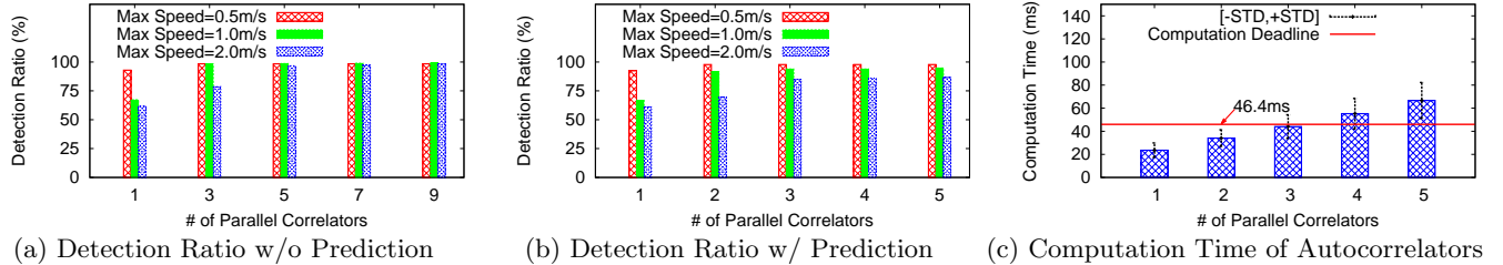
Figure 18: Parallel Autocorrelators. (a) 90+% of the tones can be detected by five parallel autocorrelators, which corresponds to offset range [L/2 - 2, L/2 + 2] (b) With predictive parallel autocorrelators, only three autocorrelators are needed. 85+% of the tones can be detected even at 2.0m/s hand movement speed. (c) Three parallel autocorrelators can still meet the computation deadline.
